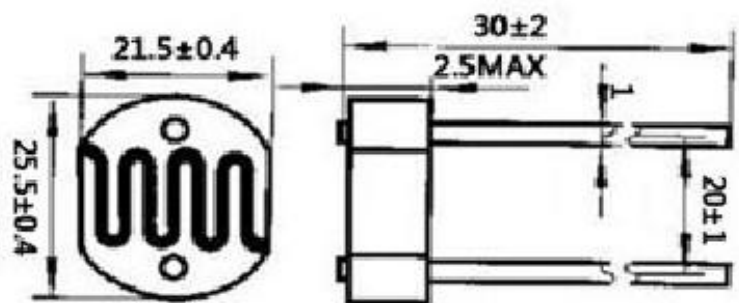
Overall dimension drawing (unit: mm)
