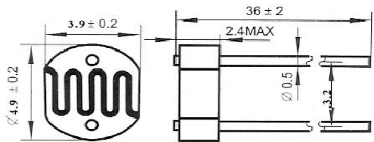
Overall dimension drawing (unit: mm)
