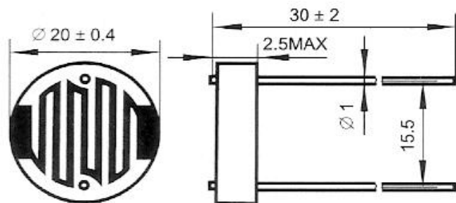
Overall dimension drawing (unit: mm)
