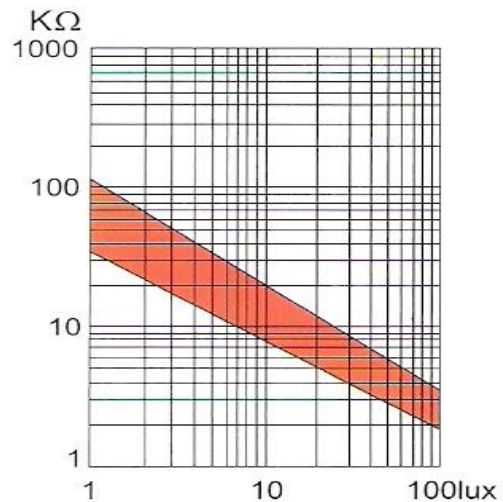
照度-电阻特性 ( Illuminance-resistance characteristics )
