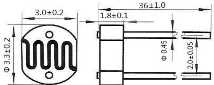
Overall dimension drawing (unit: mm)
