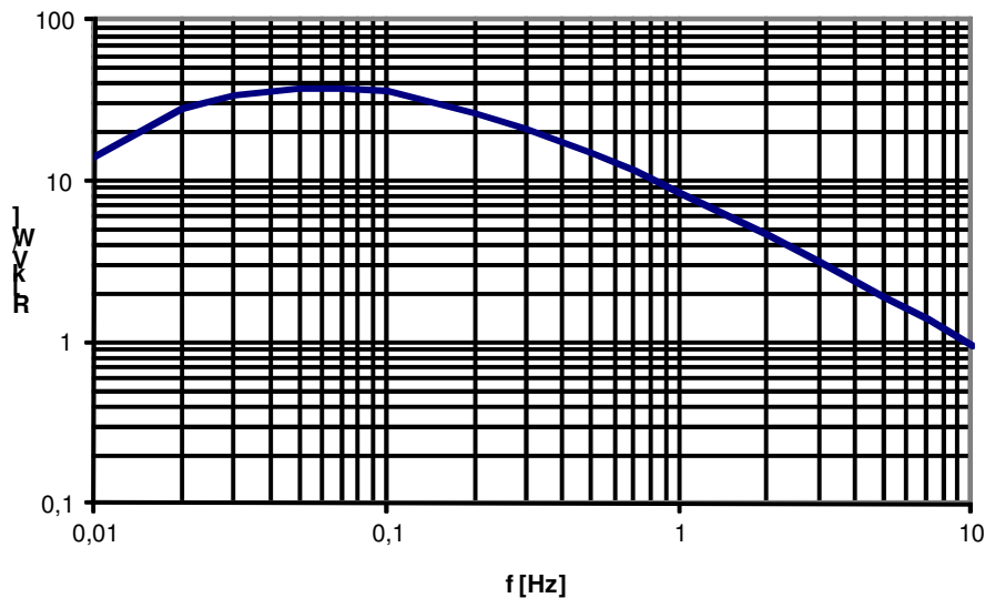
Fig. 3: Frequency response
