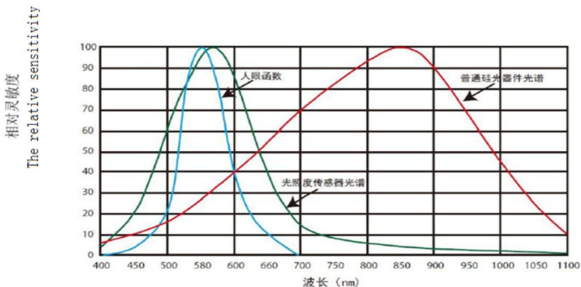
图 1-1 — Photoreceptor curve — PT850 — Visible light sensor curve
