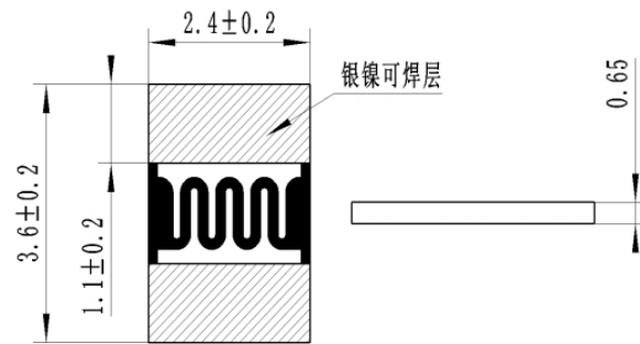
Overall dimension drawing (unit: mm)
